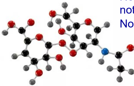
ACIDE GLUCURONIQUE
